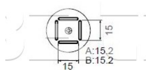
A1126B QFP 14 x 14
