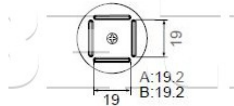
A1127B QFP 17.5 x 17.5
