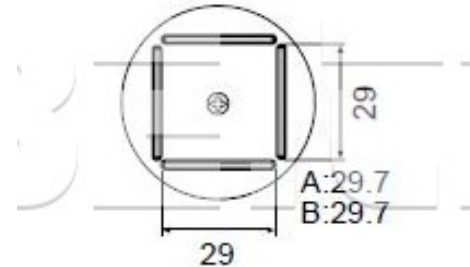
A1129B QFP 28 x 28
