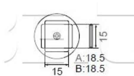
A1135B PLCC 17.5 x 17.5
