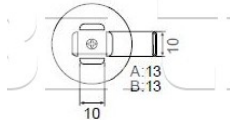
A1140B PLCC 11.5 x 11.5 (28 Pins)
