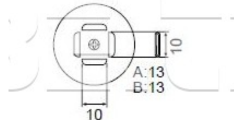
A1140B PLCC 11.5 x 11.5 (28 Pins)
