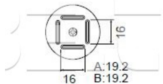
A1181B BQFP 19 x 19
